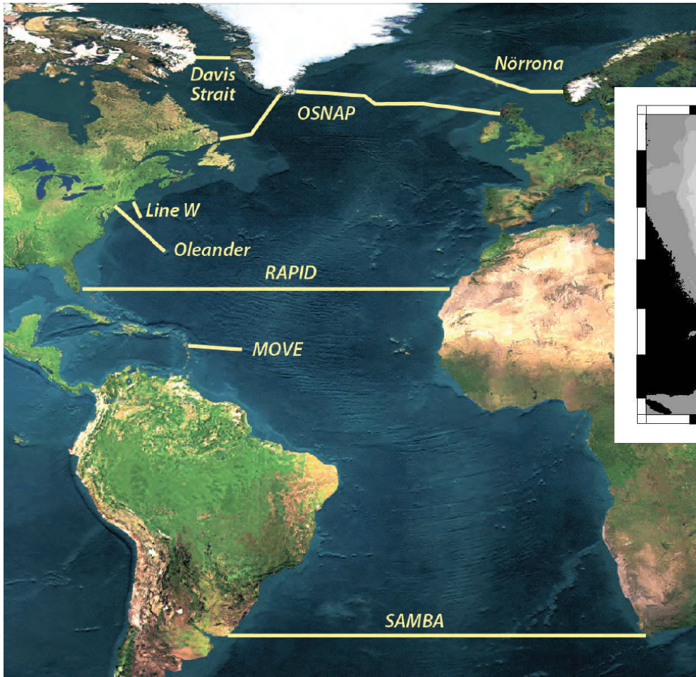
OSNAP: Overturning in the Subpolar North Atlantic
